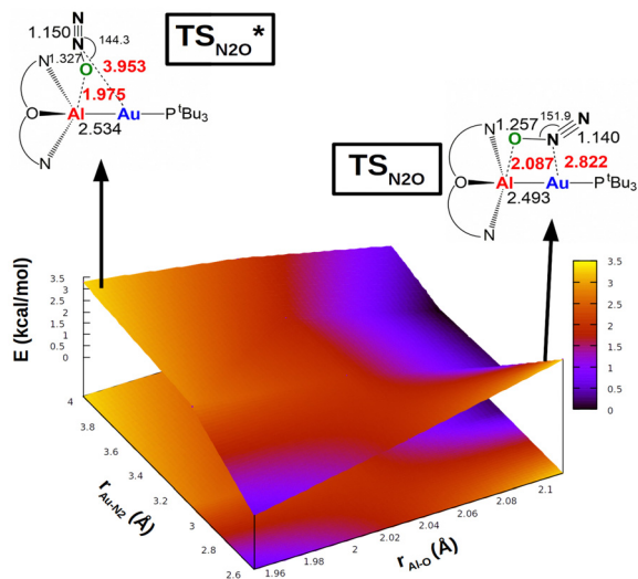
Fig. 6 Potential energy surface (PES) in the region neighbouring the transition state TS for the reaction of complex [tBu_3PAuAl(NON)] with N_2O . Insets: Position on the PES and schematic structure of TS and TS1*. Energy has been shifted in each case according to the minimum energy structure. Reproduced with permission from ref. 63 Copyright 2023, Wiley-VCH GmbH.
