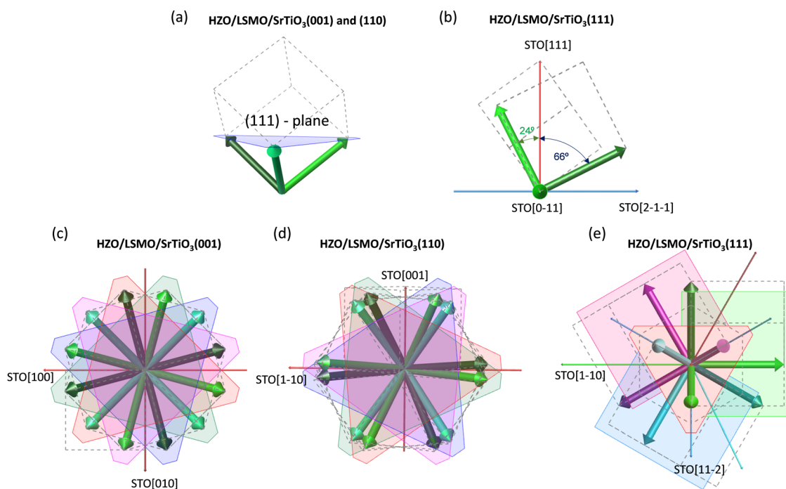
Fig. 1 (a and b) Sketch of the out-of-plane crystallographic orientation of orthorhombic HZO films grown on (a) LSMO/SrTiO 3 (001) and LSMO/SrTiO 3 (110), and (b) LSMO/SrTiO 3 (111) corresponding to one of the crystalline variants. (c–e) Sketch of all the possible in-plane directions of the polar axis of orthorhombic HZO films grown on LSMO/SrTiO 3 (001), LSMO/SrTiO 3 (110), and LSMO/SrTiO 3 (111), respectively. Axes are along the two in-plane orientations of the substrate along its edges. In (c–e) each crystalline variant is indicated by a different color.
