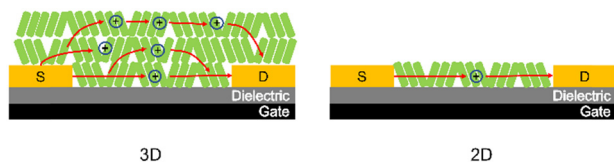
Scheme 1 Schematic illustration of charge transport in organic semiconducting multilayer (left) and monolayer (right) FETs with three-dimensional (3D) and 2D transport.
