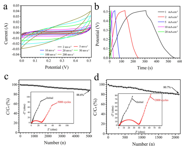
Fig. 6 The electrochemical performance of a SSS. (a) CV curves at different scan rates, (b) GCD curves at different current densities, and (c) cycle stability curve at 10 \text{ mA cm}^{-2} . (d) Cyclic stability of the SSS after 2000 bending cycles at a current density of 10 \text{ mA cm}^{-2} . Inset: Nyquist plots of the SSS.
