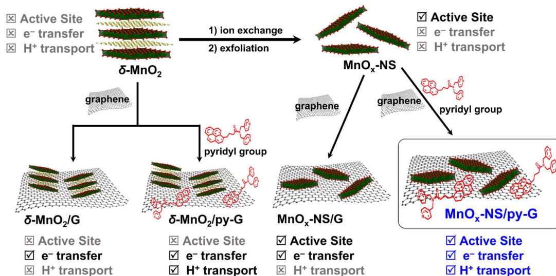
Scheme 2 Schematic illustration of the synthetic procedure of MnO_x-NS/G , MnO_x-NS/py-G , \delta-MnO_2/G , and \delta-MnO_2/py-G .
