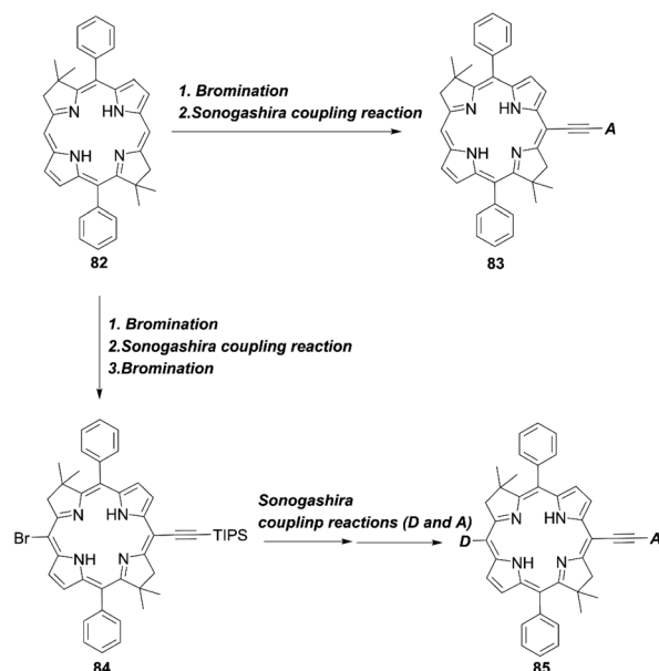
Scheme 18 Synthetic strategy for meso-functionalized bacteriochlorins.
