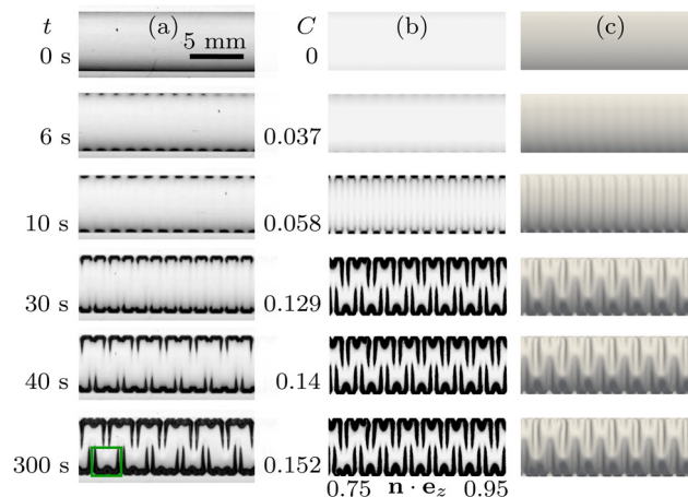
Fig. 3 Top view of (a) the time-evolving buckling patterns in the experiment, and (b) and (c) the corresponding evolution of the patterns with increasing swelling ratio C in the numerical simulations, when P = 493 Pa. The swelling ratio C is related to time t from the start of the experiment via eqn (1). The data in (b) and (c) is identical, except the colours in (b) are chosen to resemble experimental images and correspond to a grayscale contour plot of the vertical component of the unit normal \mathbf{n} to the membrane, \mathbf{n} \cdot \mathbf{e}_z , so that darker regions indicate larger membrane slopes, while the shading in (c) corresponds to illumination of the membrane by ambient light. A close-up of the region enclosed by the green box in column (a) is shown in Fig. 4(a).
