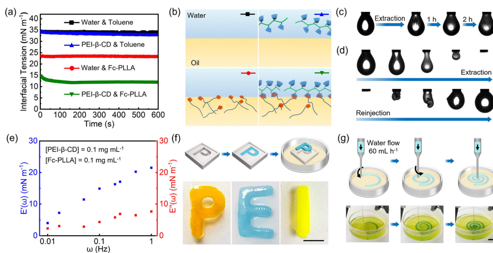
Fig. 2 (a) Time evolution of interfacial tension of different oil–water systems including water/toluene, PEI-β-CD@water/toluene, water/Fc-PLL@toluene and PEI-β-CD@water/Fc-PLL@toluene. (b) Schematics of different oil–water systems in (a). (c) Morphology evolution of the pendant droplet on the surface. (d) A series of snapshots showing the shape evolution of a pendant droplet in an extraction–re-injection process; [PEI-β-CD] = 0.1 mg mL -1 , [Fc-PLL] = 1.0 mg mL -1 . (e) Storage and loss dilatational moduli, E'(\omega) and E''(\omega) of PEIS-based interfacial assemblies, [PEI-β-CD] = 0.1 mg mL -1 , [Fc-PLL] = 0.1 mg mL -1 , \omega = 0.01 –1 Hz. (f) Schematic diagram and optical images of liquid letters “PEI” fabricated by all-liquid molding, [PEI-β-CD] = 5.0 mg mL -1 , [Fc-PLL] = 5.0 mg mL -1 . (g) Schematic diagram and optical images of the prepared liquid spiral, [PEI-β-CD] = 20 mg mL -1 , [Fc-PLL] = 20 mg mL -1 . Scale bar: 1.0 cm.
