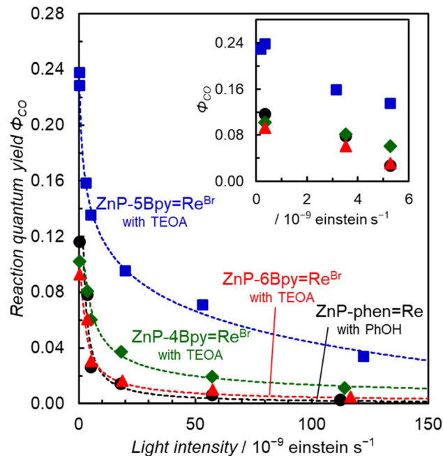
Fig. 12 Dependence of \Phi_{\text{CO}} on the irradiation light intensity (Xe lamp, \lambda_{\text{ex}} = 420 nm) for the dyads \text{ZnP-4Bpy}=\text{Re}^{\text{Br}} (green diamond), \text{ZnP-5Bpy}=\text{Re}^{\text{Br}} (blue square), and \text{ZnP-6Bpy}=\text{Re}^{\text{Br}} (red triangle) (0.05 mM) in \text{CO}_2 -saturated DMA-TEOA (4 : 1 v/v) solutions containing BIH (0.05 M), and for \text{ZnP-phen}=\text{Re} (black circle) (0.05 mM) in \text{CO}_2 -saturated DMA containing BIH (0.05 M) and phenol (0.1 M). Inset shows magnification of CO formation dependence at low light intensity.
