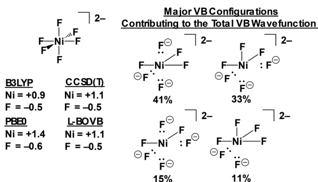
Fig. 12 Contribution of each HLSP state function to the overall valence bond wavefunction at the L-BOVB/Sapporo-DZVP-2012 level of theory (right). Mulliken charge on the nickel and fluorine centers at the PBE0/def2-QZVPP, CCSD(T)/def2-QZVPP and L-BOVB/Sapporo-DZVP-2012 levels of theory (bottom left).
