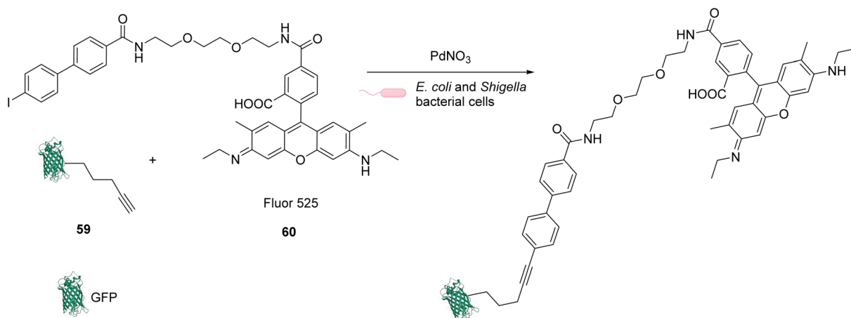
Fig. 24 Sonogashira cross-coupling inside E. coli or Shigella cells with Pd(NO 3 ) 2 as a pre-catalyst for coupling of fluorescent protein GFP with Fluor 525 and bioorthogonal labeling of toxin proteins in living pathogenic Shigella cells. 67
