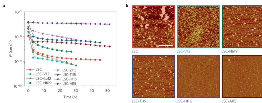
Fig. 21 (a) Oxygen surface exchange coefficient, k^{\text{eff}} , quantified from electrochemical impedance spectroscopy measurements over time at 530 °C in air, for the LSC and LSC-Me films. (b) Atomic force microscopy images of the LSC, LSC-V12, LSC-Nb19, LSC-Ti15, LSC-Hf. (Reproduced with permission from ref. 56 Copyright 2016 Nature.)
