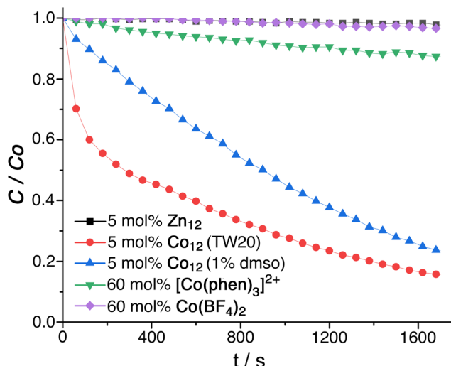
Fig. 5 Destruction of fluorescein by oxidation with peroxo-monosulfate under different sets of conditions, showing the importance of both cage-based encapsulation (red and blue lines vs. green and purple) and the importance of having \text{Co(II)} ions in the cage superstructure as redox agents for activation of peroxymonosulfate (red vs. black lines).
