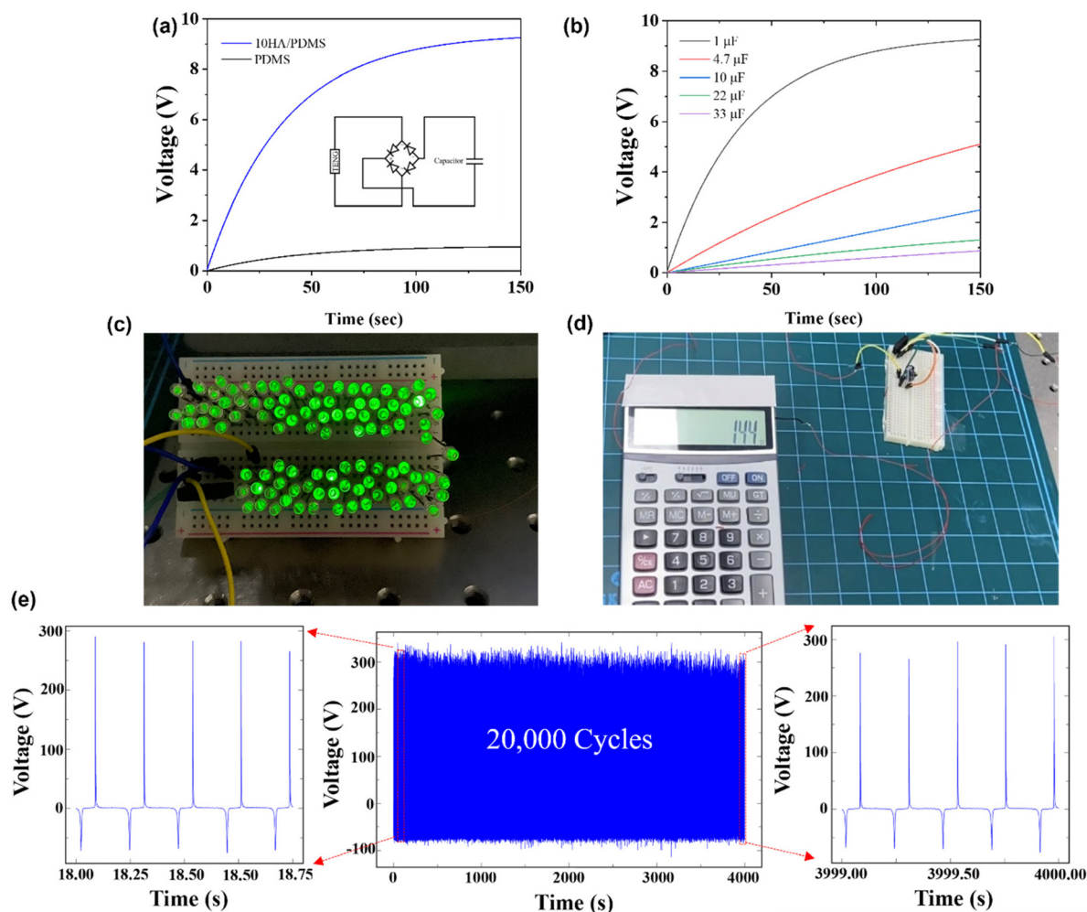
Fig. 5 (a) The charging curves of a 1\ \mu\text{F} capacitor comparing PDMS and optimal 10HA/PDMS at an input frequency of 5 Hz and an applied force of 2 N. (b) The charging curves of different capacitors with optimized 10HA/PDMS at an applied force of 2 N. (c and d) HA-TENG powering 100 LEDs or a commercial calculator. (e) Endurance test of the optimized HA-TENG for more than 20 000 cycles.
