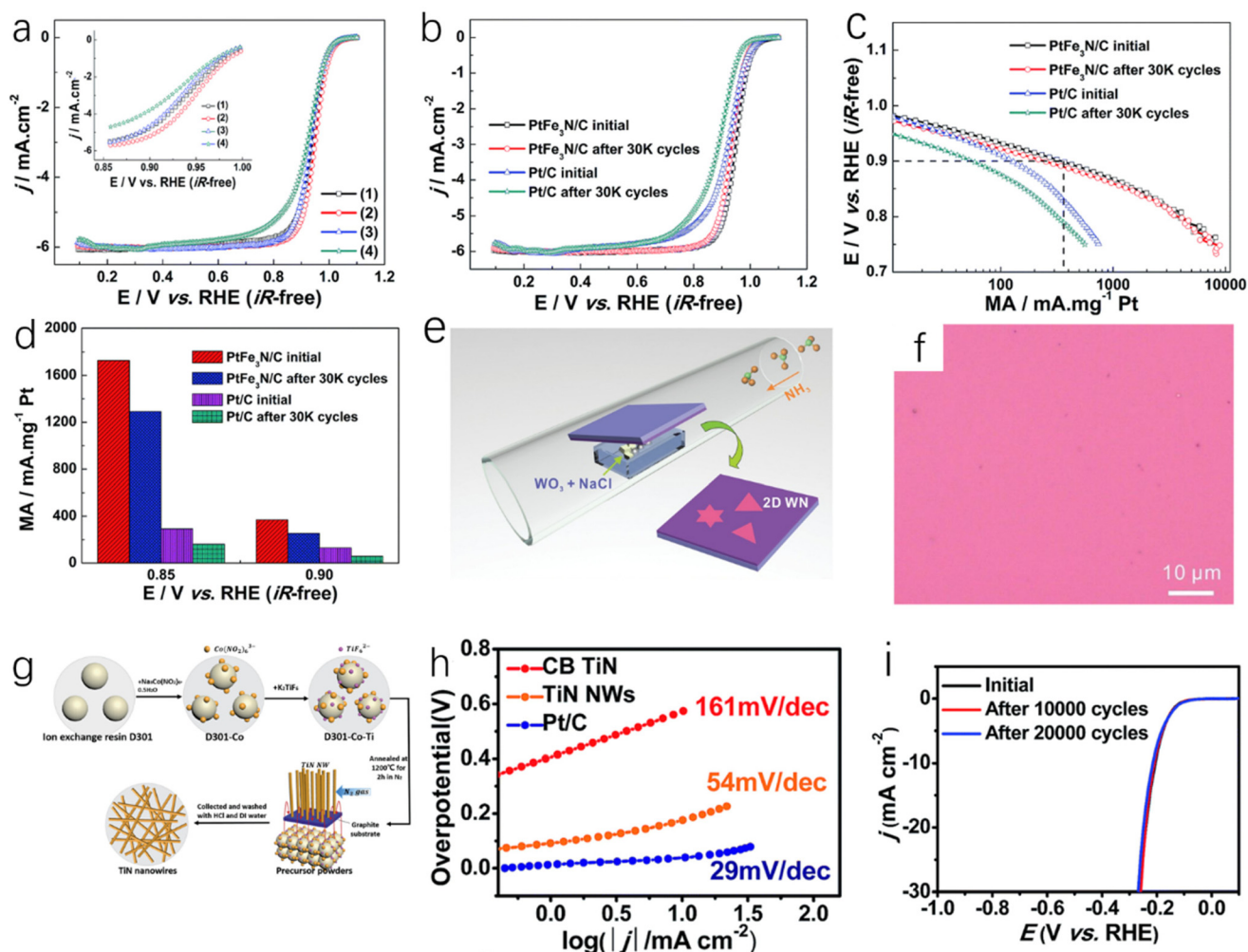
Fig. 4 (a) ORR polarization curve of the catalyst in O_2 -saturated 0.1 \text{ mol L}^{-1} \text{ HClO}_4 aqueous solution (25 °C, scanning rate 5 \text{ mV s}^{-1} , rotation speed 1600 rpm), (inset: high-magnification polarization curve); (b) ORR polarization curves of \text{PtFe}_3\text{N/C} and \text{Pt/C} catalysts before and after ADT in O_2 -saturated 0.1 \text{ mol L}^{-1} \text{ HClO}_4 aqueous solution (25 °C, scan rate of 5 \text{ mV s}^{-1} , rotation speed of 1600 rpm); (c) comparison of mass activity (MA) before and after cycling; (d) comparison of mass activity of \text{PtFe}_3\text{N/C} and \text{Pt/C} before and after cycling at 0.90 V and 0.85 V. 28 Copyright 2015, Royal Society of Chemistry; (e) a schematic CVD synthesis of ultrathin WN; (f) optical image of the product grown on \text{SiO}_2/\text{Si} substrate (without salt). 31 Copyright 2019, Wiley-VCH; (g) synthetic route of TiN NWs; (h) Tafel plots of TiN NWs, CB TiN and \text{Pt/C} electrodes; (i) the stability test of TiN NWs catalyst carried out by potential cycling, which shows the initial polarization curve and the polarization curve after 10 000 and 20 000 potential cycles. 32 Copyright 2016, Royal Society of Chemistry.
