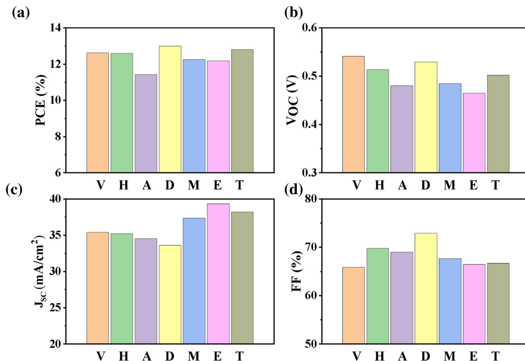
Fig. 10 (a–d) Experimental device performance values for efficiency, V_{oc} , J_{sc} , and FF for champion vacuum 25 and solution-processed CZTSSe (H, 30 A, 65 D 24 , M, 117 E, 120 and T 146 ) solar cells, respectively.
