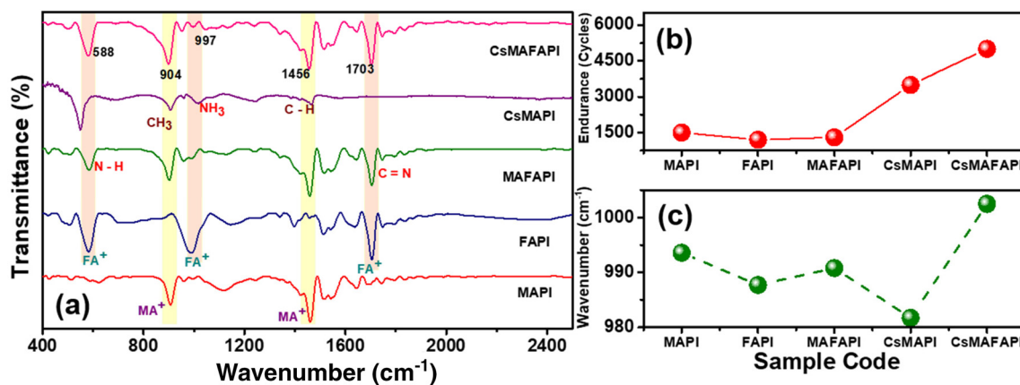
Fig. 5 (a) FTIR spectra for the MW-ST synthesized APbI 3 (A = MA + , FA + , MAFAP + , CsMA + and CsMAFA + ) metal halide perovskites with (b) the endurance cycles for the fabricated devices of configuration of Ag/APbI 3 /Ag with (c) the shift of \gamma (C-N) vibrations.
