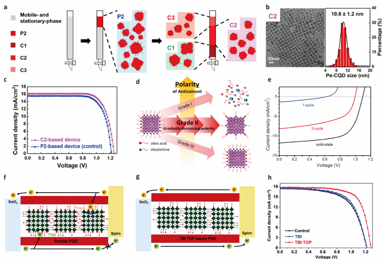
Fig. 4 Purification of the PQRDs. (a) Schematic illustration of size selection via gel permeation chromatography. (b) HR-TEM images and the size distribution histogram of the best performed PQRDs. (c) J - V curves of the control and GPC size selection-based PQRDs. (a-c) Reproduced with permission from ref. 12, Copyright 2021, American Chemical Society. (d) Schematic illustration of strategy for rational design of solvent treatment for FAPbI 3 QDs. (e) J - V curves of the devices based on FAPbI 3 after cyclic purification. (d and e) Reproduced with permission from ref. 26, Copyright 2018, Elsevier. Schematic diagrams of the charge transport in (f) control device and (g) TBI-TOP-based devices. (h) Photovoltaic performances of control, TBI-based, and TBI-TOP-based devices. (f-h) Reproduced with permission from ref. 35, Copyright 2021, Royal Society of Chemistry.
