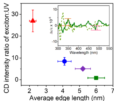
Fig. 5 Plot of the ratio of the exciton: UV region CD intensity versus the NP edge length for 2 nm (red), 4 nm (blue), 5 nm (purple), and 6 nm (green) NPs. Inset shows a representative CD spectrum with the UV and the exciton intensity marked in orange and pink respectively.
