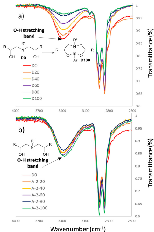
Fig. 6 FTIR overlays of (a) epoxy-amine-dioxazaborocane materials (D0–D100, inset: representative molecular structure of D0 and D100) and (b) epoxy-amine thermoset materials (A 2 -20–A 2 -100, inset: representative molecular structure).
