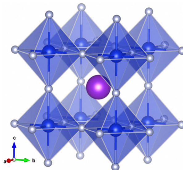
Fig. 1 Polyhedral view for the crystalline structure of all-inorganic lead-free fluoride perovskite \text{ABF}_3 ( \text{A} = \text{Na}, \text{K} and \text{B} = \text{Si}, \text{Ge} ) with a space group \text{Pm}\bar{3}\text{m} . The purple, blue and gray balls represent the A, B and F atoms, respectively.
