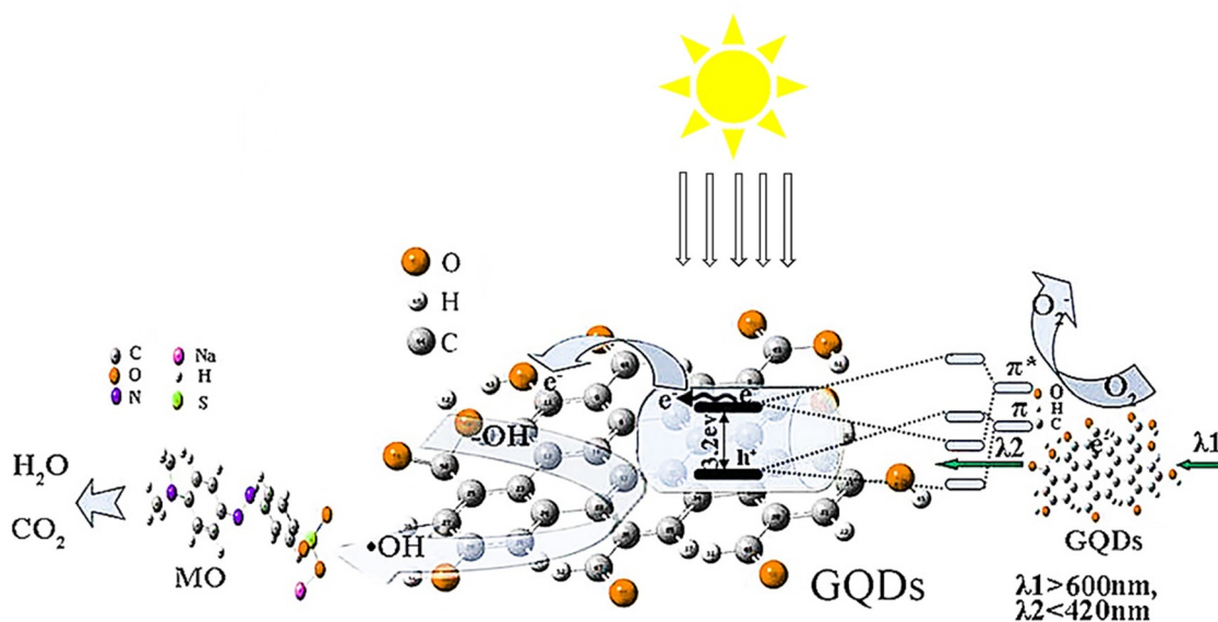
Fig. 13 The schematic of the improved light-driven photocatalysis of GQD/TiO 2 -NT composites. Reproduced with permission from ref. 110. Copyright (2016) Elsevier.
