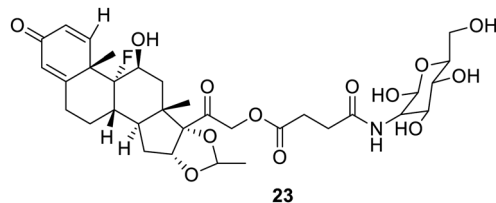
Fig. 15 Triamcinalone acetamide substituted with succinate and glucosamines.
