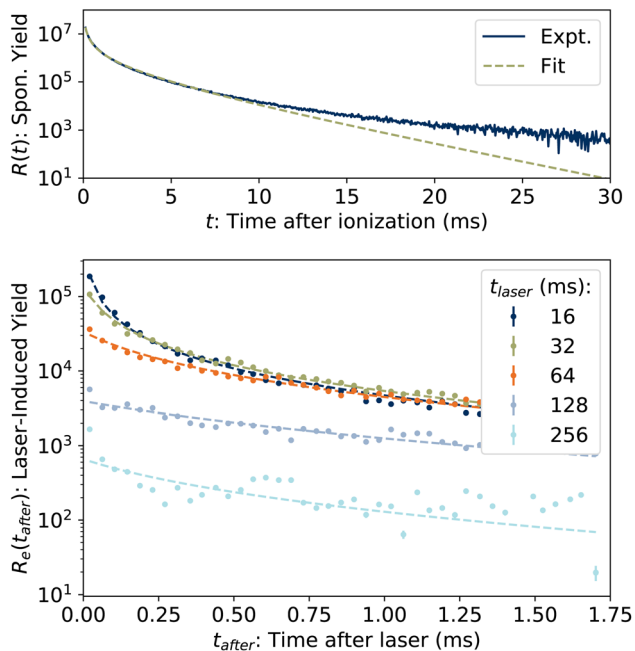
Fig. 2 (Top) Spontaneous dissociation rate R(t) , fit of eqn (4). (Bottom) Examples of laser-induced dissociation rates R_e(t_{\text{after}}) with fits of eqn (8).
