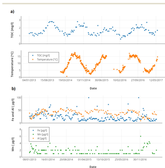
Fig. 3 WTW outlet treated water quality from discrete samples, January 2013 to May 2017 a) TOC and temperature b) iron, aluminium and manganese.
