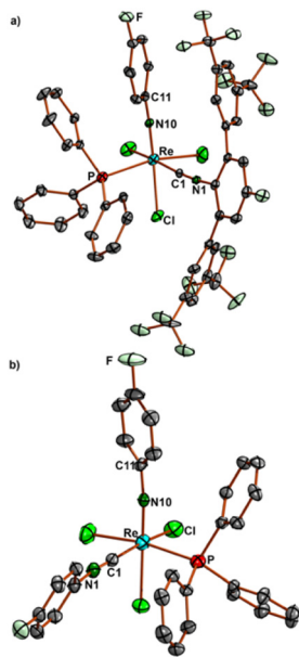
Fig. 7 Molecular structures of a) fac -[Re(NPh)Cl 3 (PPh 3 )(CNAr DarF2 ) 2 ] ( 11 ) and b) mer -[Re(NPh)Cl 3 (PPh 3 )(CNPhPF 2 ) 2 ] ( 12 ). Selected bond lengths and angles for 11 : Re–N10 1.721(43), Re–P 2.4494(9), Re–C1 2.022(3), C1–N1 1.151(4) Å; Re–N10–C11 170.4(2), and Re–C1–N1 174.6(43)°; selected bond lengths and angles for 12 : Re–N10 1.705(4), Re–P 2.470(2), Re–C1 2.024(6), C1–N1 1.156(7) Å; Re–N10–C11 172.9(4), and Re–C1–N1 176.9(5)°.
