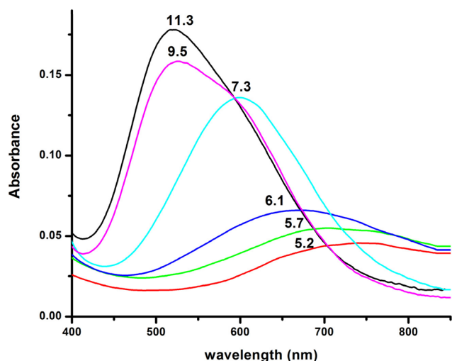
Fig. 8 Visible absorption spectra of the solutions of Cu(II) and R1 (Cu(II) : R1 = 1 : 1.2, T = 298 \text{ K} , I = 0.1 ( \text{KNO}_3 )), recorded at the indicated pH values.
