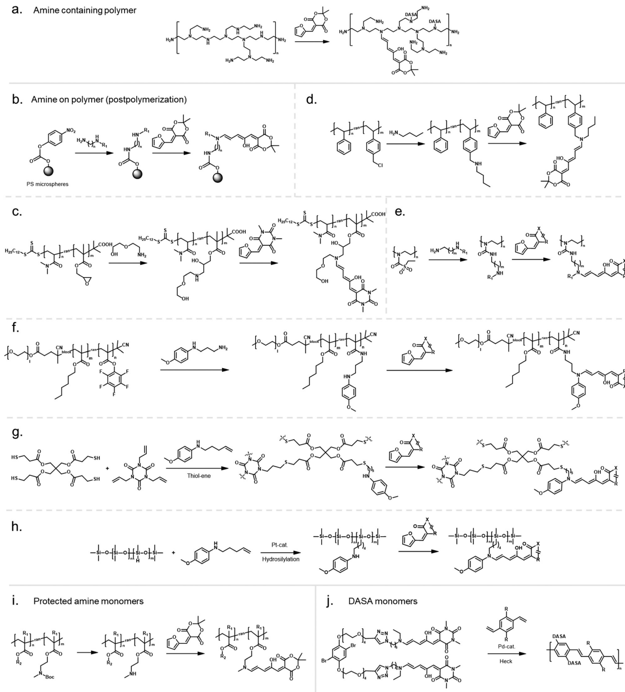
Fig. 10 Different strategies for DASA conjugation to polymers via the donor moiety and polymerization of DASA monomers. (a) Utilization of amines inherently present in a polymer backbone, e.g. , PEI, for DASA formation. In most examples, amine conjugation was performed via postpolymerization followed by DASA formation by reaction with furan adducts. Different functional monomers or functional groups were used to introduce secondary amines postpolymerization, such as (b) carbonates, e.g. , p -nitrophenyl carbonate (c) epoxide groups, e.g. , glycidyl methacrylate, (d) alkyl halides, e.g. , 4-vinylbenzyl chloride (e) sulfonyl groups, or (f) activated esters, e.g. , pentafluorophenyl(meth)acrylate. (g) Amine functionalization of thiol-ene resins during the network formation step by using alkene-functional amines. (h) Amine functionalization of PDMS via hydrosilylation with alkene-functional amines. (i) Copolymerization of protected alkylamine (meth)acrylate derivatives to introduce the amine functionality during the polymerization step. (j) Only reported example of polymerization of DASA monomers involving Heck coupling of dibromobenzene DASA-functionalized monomers with a divinylbenzene derivative.
