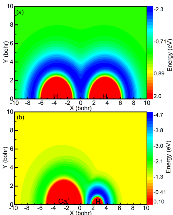
Fig. 3 (a) Contour plot for a \text{Ca}^+ ion moving around a \text{HH} molecule fixed at R_{\text{HH}} = 7.32 bohr and lying along the x-axis. (b) Color plot for a H atom moving around a \text{CaH}^+ molecule ion fixed at R_{\text{CaH}} = 5.06 bohr. The dissociation limit of the \text{CaH}_2^+ molecule ion is set as the zero point of potential energy.
