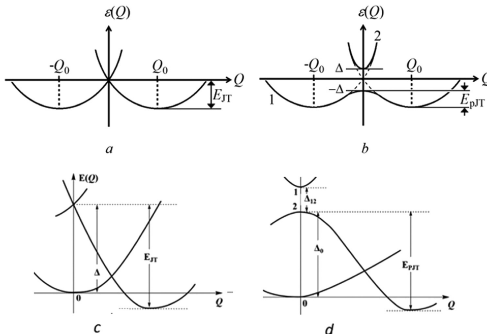
Fig. 1 Illustration of the definition of the four types of electronic configurations causing the four kinds of Jahn–Teller effects. For simplicity, in all four cases only one symmetrized coordinate Q of the low-symmetry nuclear displacements from the reference high-symmetry configuration at Q = 0 is shown, E_{JT} and E_{PJTE} are the JTE stabilization energies, and \Delta denotes energy gaps. (a) In the case of proper JTE the system is unstable, it has no minimum of the adiabatic potential energy surface (APES) at the point of electronic degeneracy Q = 0 , but it may be stable in the distorted configurations at \pm Q_0 . (b) The pseudo-JTE (PJTE) case: there is no degeneracy at Q = 0 , but the system is unstable (the curvature K of the ground-state APES is negative) due to the pseudodegeneracy caused by strong vibronic coupling F to low-lying excited states at \Delta < F/K (see the text). (c) Hidden-JTE: there is neither degeneracy nor pseudodegeneracy in the ground state of the system, but there is a relatively low-lying excited state that has a JTE, which is so strong, E_{JT} > \Delta , that it penetrates the high-symmetry ground state, producing a global minimum with a distorted configuration. (d) Hidden-PJTE: the same situation as in the hidden-JTE, but the intervening excited state has a strong PJTE, instead of the JTE.
