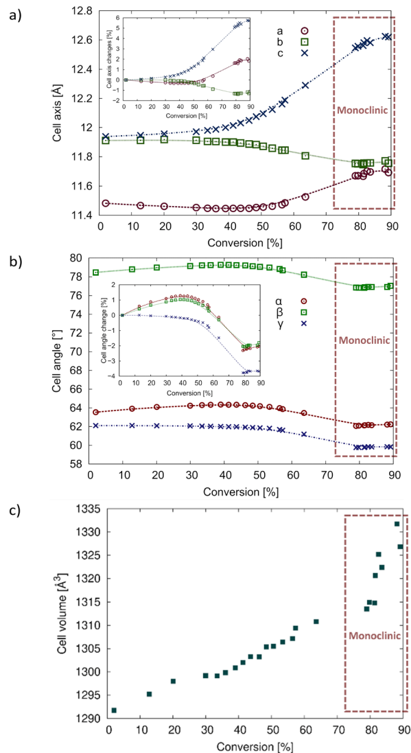
Fig. 9 Changes in unit cell parameters with degree of conversion for the crystal reacted at 20\text{ }^\circ\text{C} . The points that are enclosed with a red rectangle were transformed from the monoclinic unit cell back to the triclinic cell of the CT (see text for details). (a) Changes in a - c with the inset graph showing the percent change; (b) change in cell angles with the inset graph showing the percent change; (c) change in cell volume. Plots of the 40\text{ }^\circ\text{C} data are superimposed on this data in Fig. S2 in the ESI†
