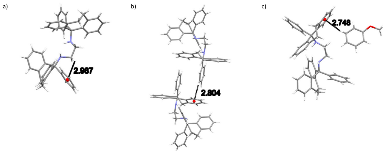
Fig. 5 Depiction of a) one of the intramolecular (host)C–H \cdots\pi (host), b) the only intermolecular (host)C–H \cdots\pi (host) and c) the only intermolecular (guest)C–H \cdots\pi (host) interactions in 2(H2)·3(ANI).
