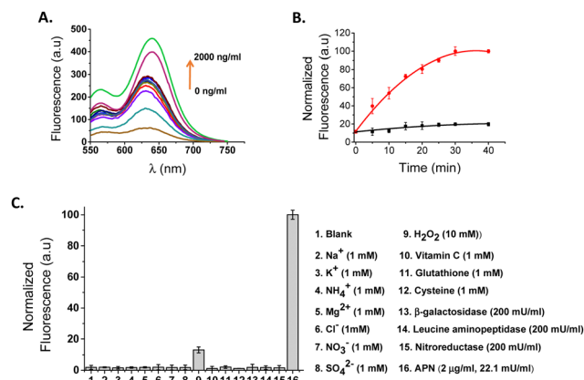
Fig. 3 (A) Fluorescence emission spectra of NB-ALA (20 \mu\text{M} ) in aqueous solution (H 2 O–DMSO 99:1 v/v, pH 7.4) in the presence of different concentrations of APN enzyme (0–2000 ng mL -1 ). (B) Fluorescence of NB-ALA in (H 2 O–DMSO 99:1 v/v, pH 7.4) at different time points in the absence (black curve) and in the presence of APN enzyme (2 \mu\text{g mL}^{-1} ) with an activity of 22.1 mU mL -1 (red curve). Error bars are expressed as 3 \sigma for three independent experiments. (C) Selectivity of NB-ALA . (H 2 O–DMSO 99:1 v/v, pH 7.4). NB-ALA (20 \mu\text{M} ) was incubated with the following interferents.
