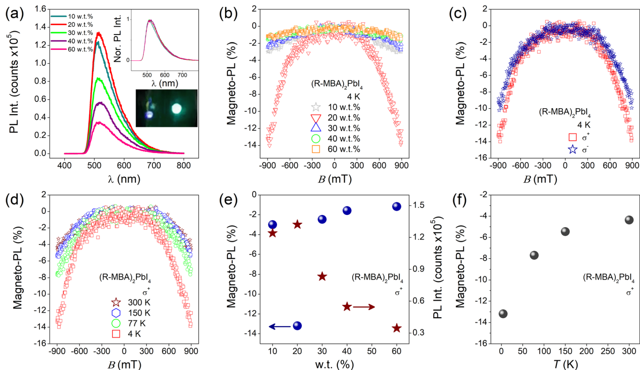
Fig. 1 (a) Experimental results of steady state photoluminescence spectra at room temperature for the (R-MBA)_2PbI_4 thin films prepared by the precursor solutions with different weight percentages (wt%), such as 10 wt%, 20 wt%, 30 wt%, 40 wt%, and 60 wt%. The upper inset plot shows the normalized spectra for the samples. The lower inset image is the photographic picture for the luminescence in the measurement. (b) The wt% dependence of the magneto-PL (%) at 4 K for (R-MBA)_2PbI_4 . (c) The measurements of magneto-PL (%) due to the left and right circularly polarized photoexcitation ( \sigma^+ and \sigma^- ) at 4 K for (R-MBA)_2PbI_4 . (d) The temperature dependence of magneto-PL (%) for (R-MBA)_2PbI_4 . (e) and (f) show the extracted values for the wt% and temperature-dependent magneto-PL (%). The photoexcitation wavelength is set to be 405 nm for all the measurements.
