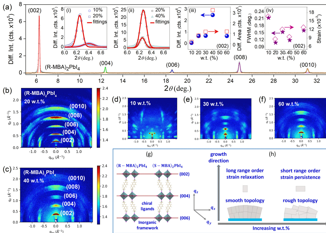
Fig. 3 (a) The XRD spectrum for the (R\text{-MBA})_2\text{PbI}_4 polycrystalline film (20 wt%). The red solid lines are the fitting curves. The insets (i and ii) are the zoom-in plots for the (002) diffracted bands of the spectra. (b–f) The GIWAXS patterns for the (R\text{-MBA})_2\text{PbI}_4 polycrystalline thin films with 20 wt%, 40 wt%, 10 wt%, 30 wt% and 60 wt%, respectively. (g and h) Pictorial descriptions of the chiral perovskite crystalline structures, out-of-plane orientation and the crystal growth mode. (R\text{-MBA})_2\text{PbI}_4 and (S\text{-MBA})_2\text{PbI}_4 possess a mirror symmetry.
