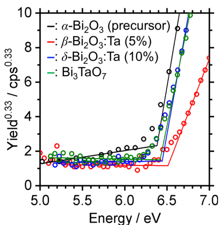
Fig. 8 Photoelectron spectra in air (PESA) of \alpha - \text{Bi}_2\text{O}_3 (precursor), \beta - \text{Bi}_2\text{O}_3 :Ta (5%), \delta - \text{Bi}_2\text{O}_3 :Ta (10%), and \text{Bi}_3\text{TaO}_7 .
