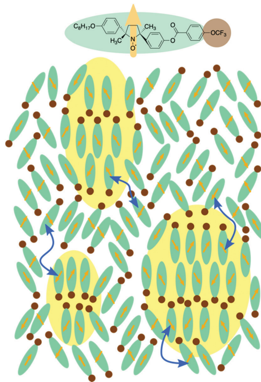
Fig. 7 Molecular orientations in and out of the cybotactic clusters. Molecules of (±)- 3 have the trifluoromethyl group (brown circles) and electron spins of nitroxide radical moieties (orange arrows). The molecules move into and out of the yellow-colored cybotactic clusters. Blue double-headed arrows denote the molecular exchange inside and outside the cybotactic clusters.
