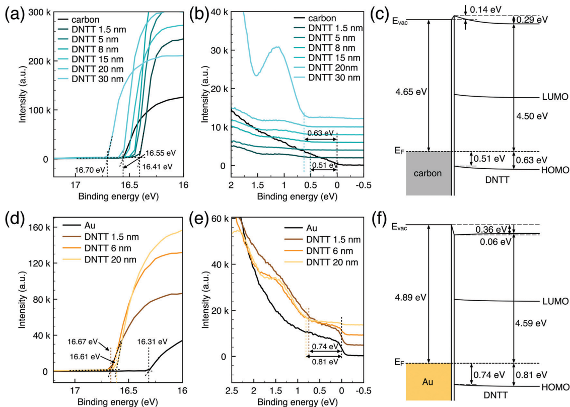
Fig. 6 (a) XPS spectra and (b) valence region of DNTT deposited on carbon for increasing coverage by the UPS. (c) Schematic energy level diagram of the DNTT/carbon interface. (d) XPS spectra and (e) valence region of DNTT deposited on Au for increasing coverage by the UPS. (f) Schematic energy level diagram of the DNTT/Au interface.
