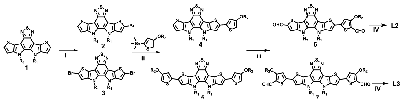
Scheme 1 Synthetic routes to L2 and L3 . (i) NBS, THF, 0 °C; (ii) (4-((2-hexyldecoyl)oxy)thiophen-2-yl)trimethylstannane, Pd(PPh 3 ) 4 , toluene, reflux; (iii) POCl 3 , 1,2-dichloroethane, DMF, 80 °C; (iv) 2-(5,6-difluoro-3-oxo-2,3-dihydro-1H-inden-1-ylidene)malononitrile, pyridine, CHCl 3 , rt.
