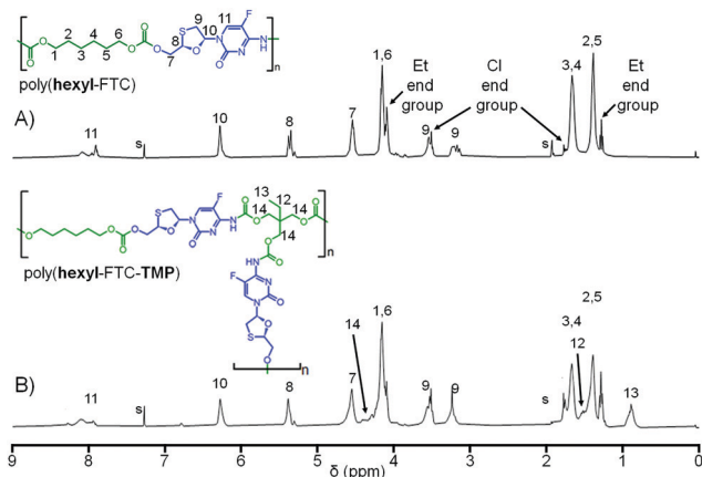
Fig. 4 Comparative 1 H nuclear magnetic resonance spectra (CDCl 3 ) of (A) linear poly(hexyl-FTC); and (B) branched poly(hexyl-FTC-TMP). Resonances identified for ethyl carbonate end groups, intentionally created to consume unreacted chloroformate chain ends, and alkyl chloride end groups derived from degradation of chloroformate monomers.
