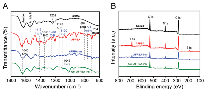
Fig. 1 FTIR and XPS analysis of glucose-responsive insulin-releasing hydrogels. (A) FTIR spectra from 1800 to 600 cm -1 , and (B) XPS wide spectra during the preparation of hydrogels.
