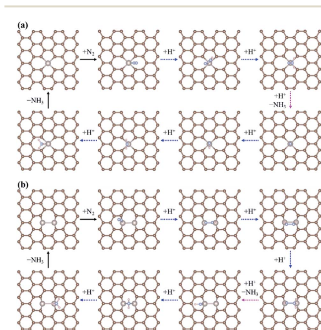
Fig. 2 The optimized geometric structures of N_2RR intermediates along the most favourable reaction pathway on (a) the Ru_1 SAC and (b) the homo- Ru_2 DAC.
