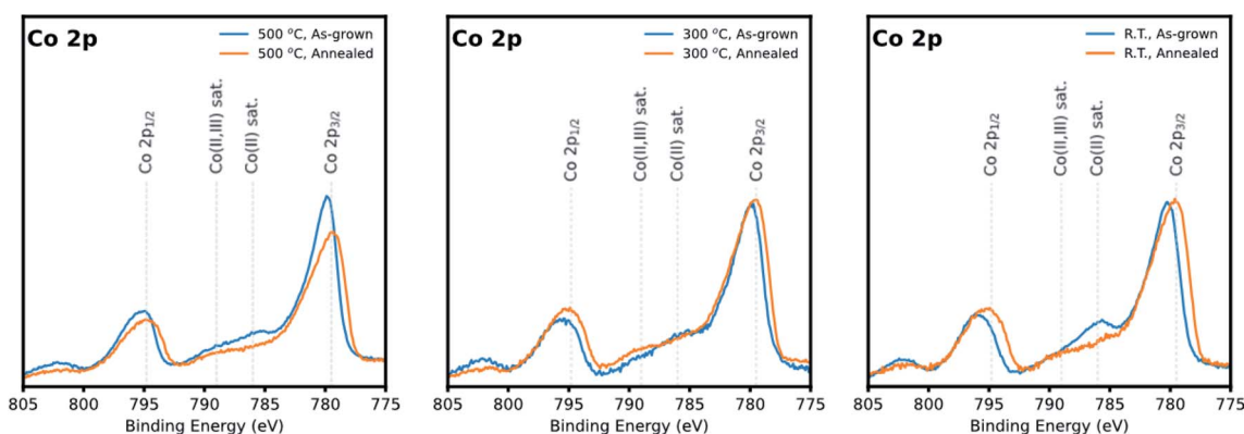
Fig. 5 X-ray photoelectron spectra of Co 2p of the LSC nanostructured films grown at 500 °C, 300 °C, and R.T. As-grown films and annealed films are depicted in blue and orange, respectively.
