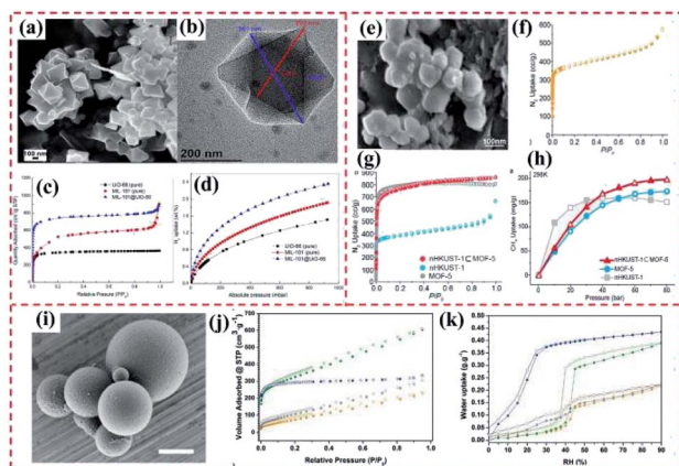
Fig. 22 (a) SEM and (b) TEM image of the core-shell nanocrystals. (c) N_2 sorption isotherms, and (d) H_2 sorption isotherms for the desolated MIL-101 (pure), UiO-66 (pure) and core-shell MIL-101@UiO-66 hybrid samples. Reproduced from ref. 18 with permission from Elsevier, Copyright 2014. (e) SEM image of nHKUST-1. (f) N_2 gas-adsorption isotherm of nHKUST-1. (g) N_2 gas adsorption isotherms of the MOF-5, nHKUST-1, and nHKUST-1 \subset MOF-5 samples. (h) Gravimetric adsorption uptake capacity of nHKUST-1 \subset MOF-5, MOF-5, and nHKUST-1 for methane. Reproduced from ref. 66 with permission from the American Chemical Society, Copyright 2015. (i) FESEM images of UiO-66-NH 2 @COF-TAPB-BTCA beads. (j) N_2 adsorption isotherms for UiO-66-NH 2 (blue), COFTAPB-BTCA beads (orange), physical mixture of these two components (grey), and UiO-66-NH 2 @COF-TAPB-BTCA beads (green). (k) Water adsorption isotherms for UiO-66-NH 2 (blue), COF-TAPBBTCA beads (orange), physical mixture of these two components (grey), and UiO-66-NH 2 @COF-TAPB-BTCA (green). Reproduced from ref. 17 with permission from Wiley, Copyright 2019.
