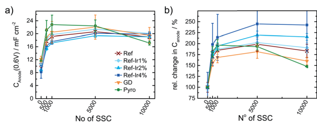
Fig. 8 (a) Change in capacitance and relative change in capacitance as a function of the number of SSC cycles applied to the catalysts. Values extracted from CV measurements in N_2 saturated 0.1\text{ M H}_2\text{SO}_4 .
