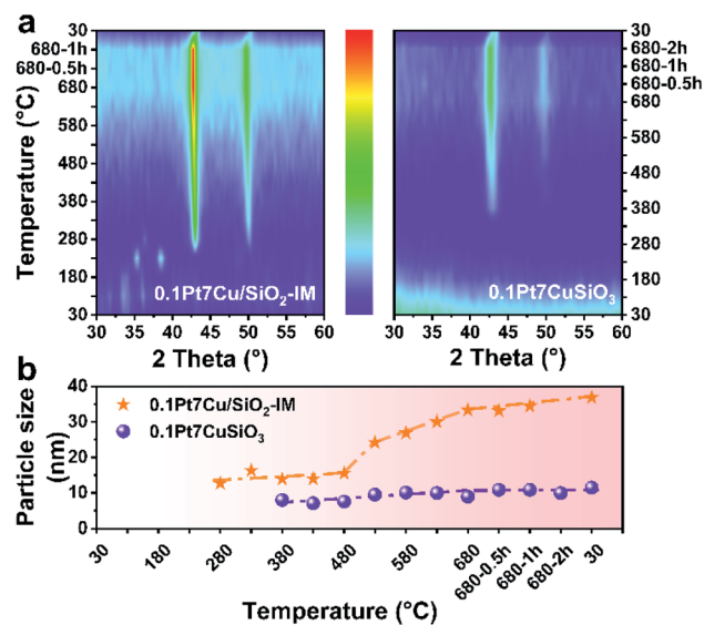
Fig. 1 (a) In situ XRD patterns of 0.1\text{Pt}7\text{Cu}/\text{SiO}_2\text{-IM} and 0.1\text{Pt}7\text{CuSiO}_3 under a reductive atmosphere. (b) The evolution of the size of PtCu NPs versus temperature for reduction of 0.1\text{Pt}7\text{Cu}/\text{SiO}_2\text{-IM} and 0.1\text{Pt}7\text{CuSiO}_3 in 10 vol% \text{H}_2/\text{Ar} .
