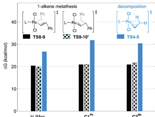
Fig. 3 Barriers to 1-alkene metathesis (via TS8-9 and TS9-10' ) or \beta -H elimination (via TS4-5 ). Free energies are given relative to the unsubstituted metallacyclobutane 4 .
