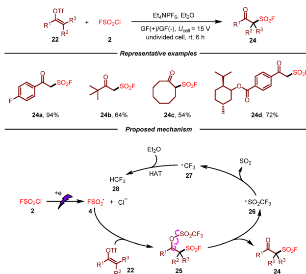
Scheme 4 Electrochemical synthesis of β-keto sulfonyl fluorides via radical fluorosulfonylation of vinyl triflates.
