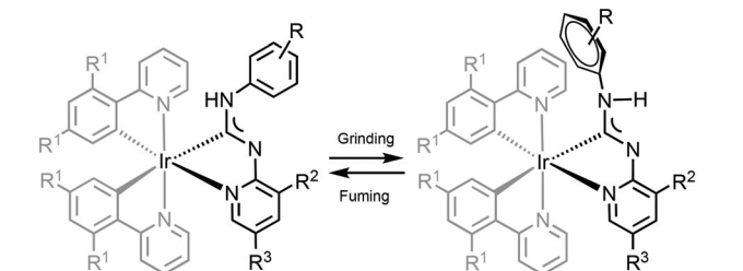
Scheme 6 (Top): preparation of 48–53 ; (bottom): proposed mechanochromic change of the Ar orientation responsible for the observed change in the emission properties of diaminocarbene complexes. 49
