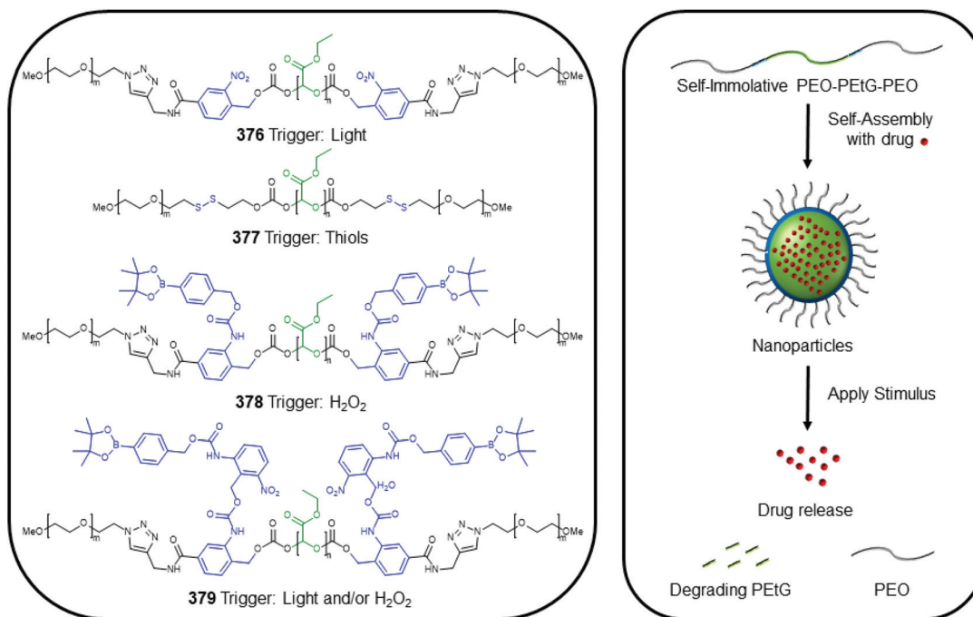
Scheme 99 The structures of the PtEtG-PEG block copolymers 376–379 that could be triggered via exposure to light, thiols or hydrogen peroxide and a schematic illustrating the self-assembly of nanoparticles plus the mode of payload delivery post application of the key stimulus. 369
