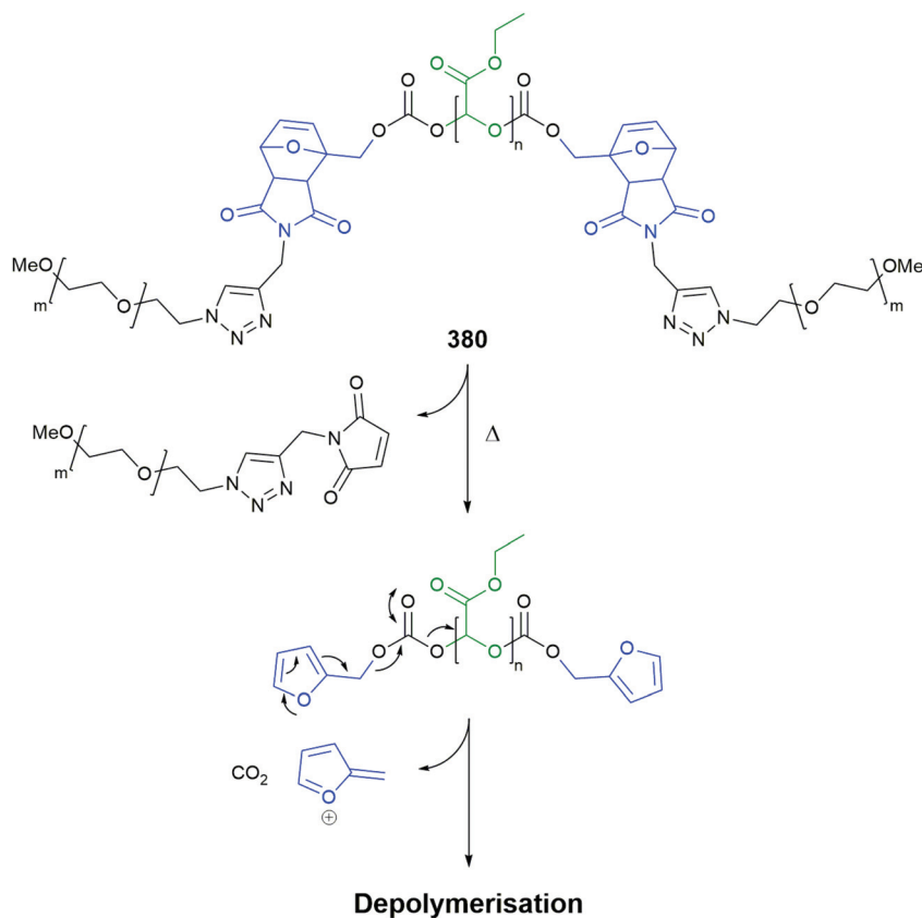
Scheme 100 The PEG-PtEtG-PEG block copolymer 380 reported by Gillies and co-workers that featured thermally degradable cycloadducts at the polymer block junctions. 175
