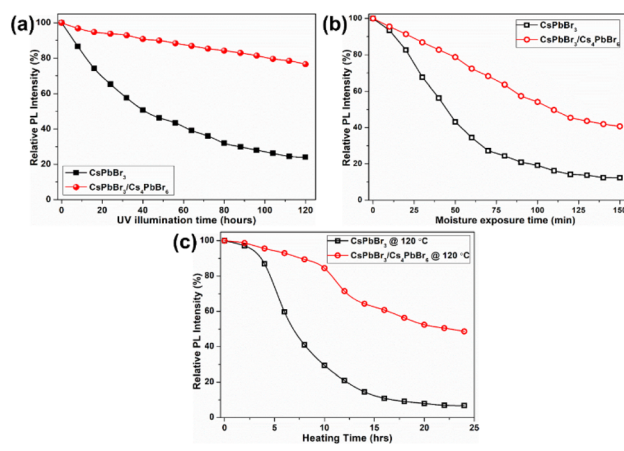
Fig. 8 (a) UV irradiation test, (b) moisture resistance test, and (c) thermal tolerance test for CsPbBr 3 NCs and dual-phase CsPbBr 3 /Cs 4 PbBr 6 MCs conducted by monitoring their emission trends at 365 nm excitation.
